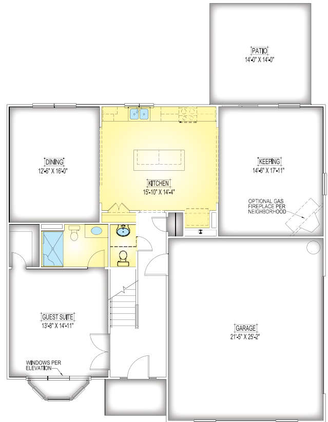
MAIN LEVEL - OPTIONAL GUEST SUITE
