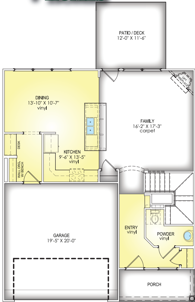
MAIN LEVEL
