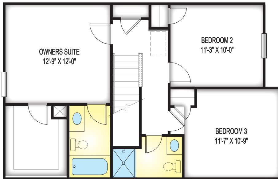
SECOND LEVEL
