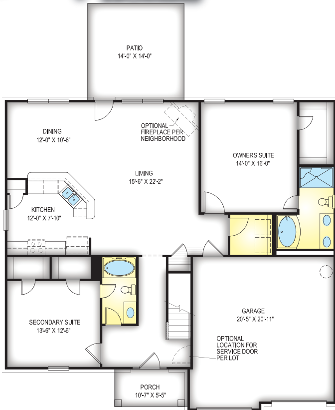
ELEVATION A MAIN LEVEL
