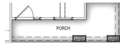
PORCH @ ELEV. C
